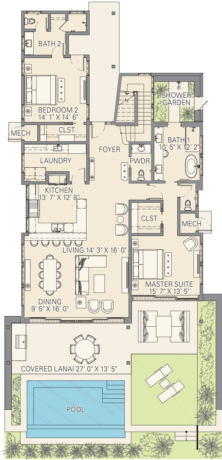
1ST FLOOR / MAIN LEVEL
