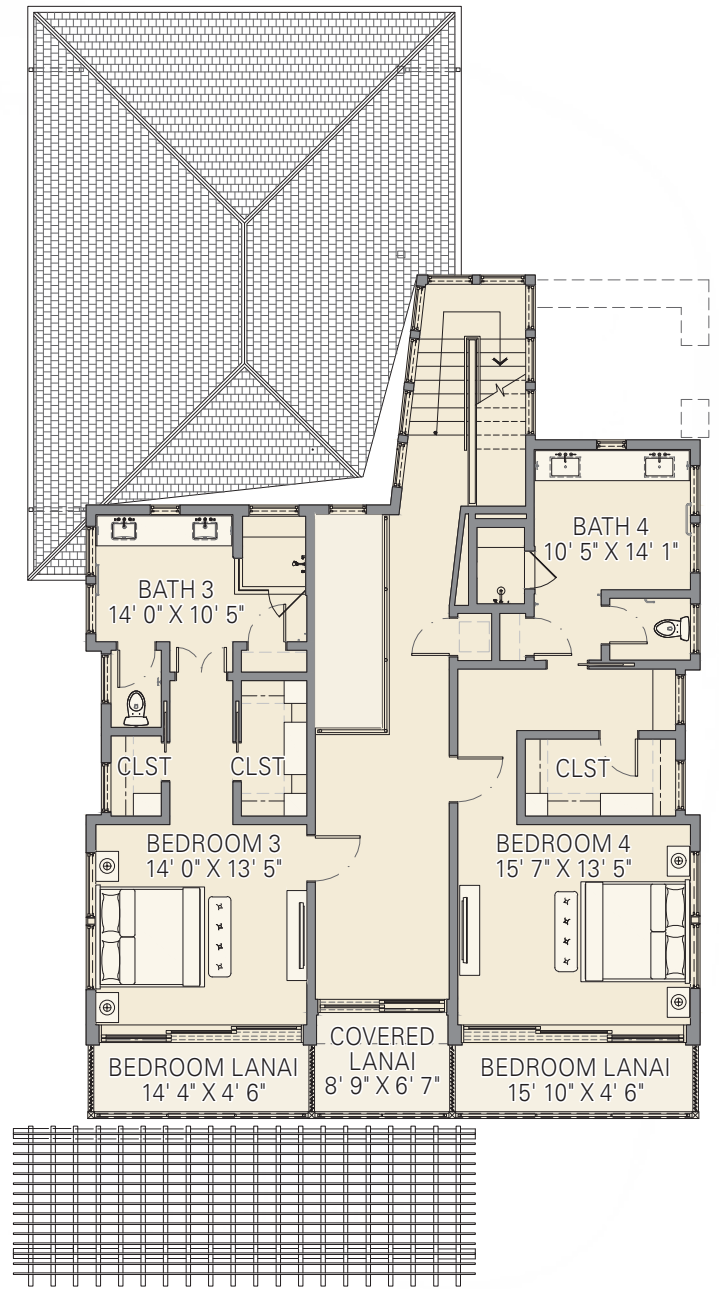
2ND FLOOR / UPPER LEVEL
