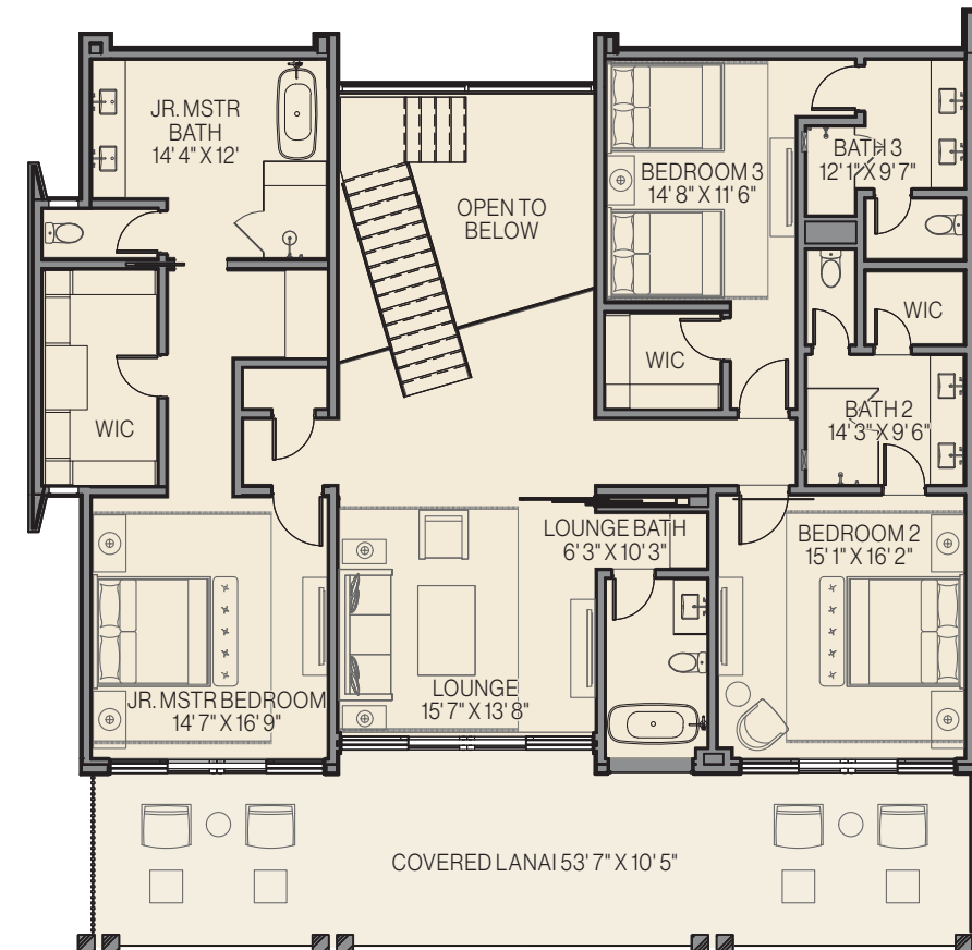
UNIT A, 2ND FLOOR / UPPER LEVEL
